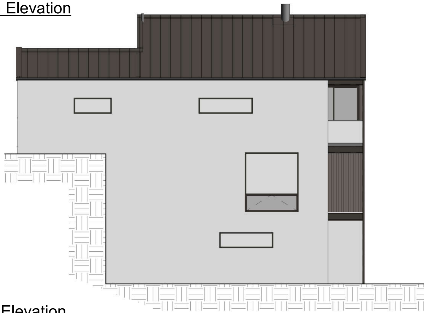
Units 9, 10 & 11 Elevations
