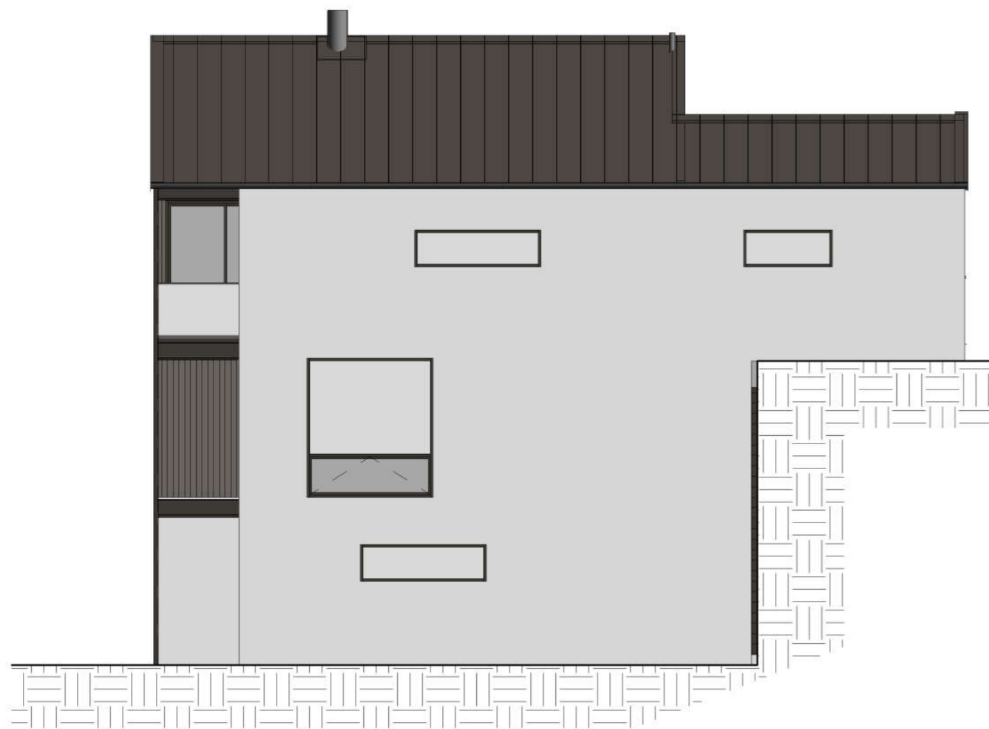
East Elevation
